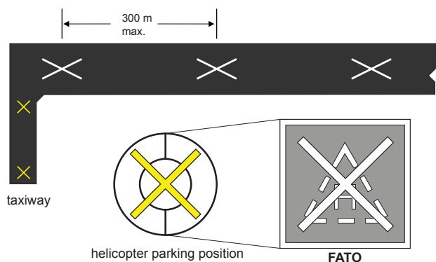
Figure 5.11—Closed Markings
