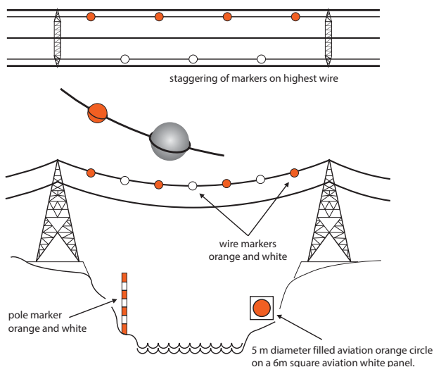
Figure 6.4—Markers for Cable Span
