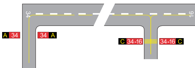
Figure 5.14—Examples of Runway Designation Signs
