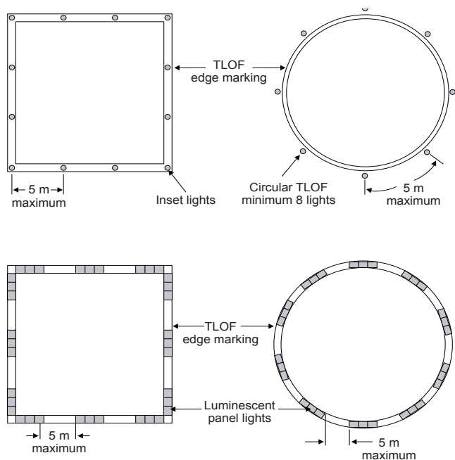
Figure 7.16—Examples of TLOF Lighting
