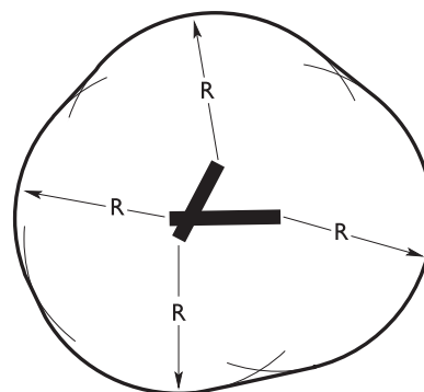
Figure 9.11—Visual Manoeuvring (Circling) Area
