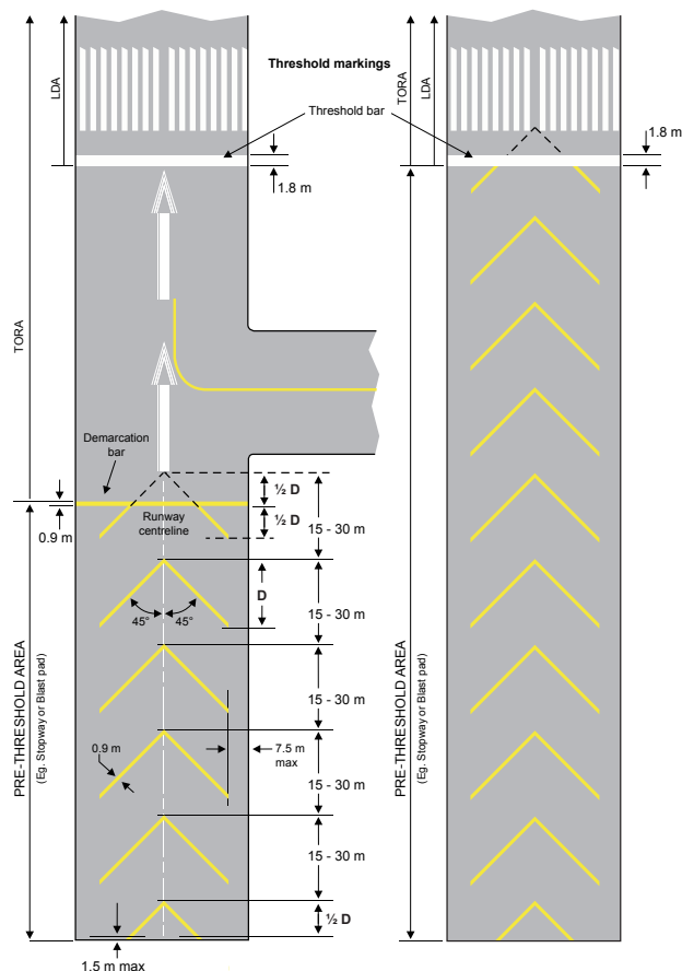
Figure 5.6—Stopway Markings
