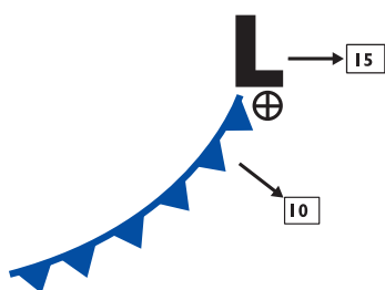
Figure 4.4(b)—Synoptic Features
