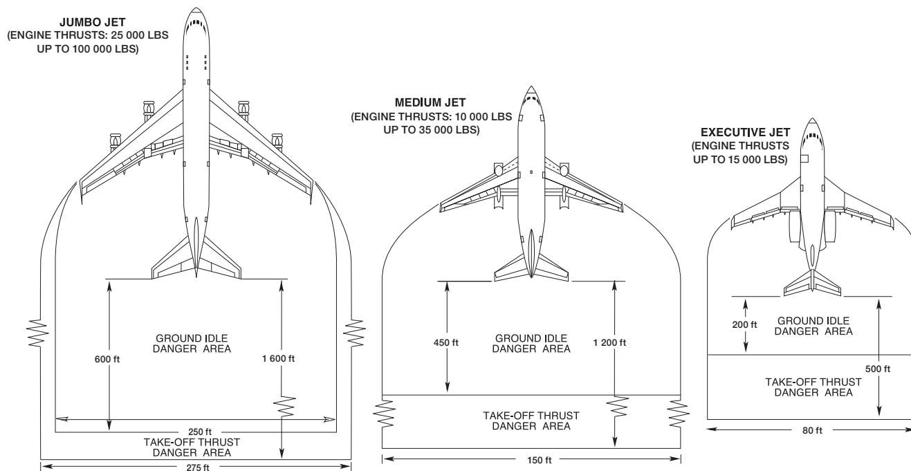
Figure 1.2—Jet Blast Danger Areas (Not To Scale)
