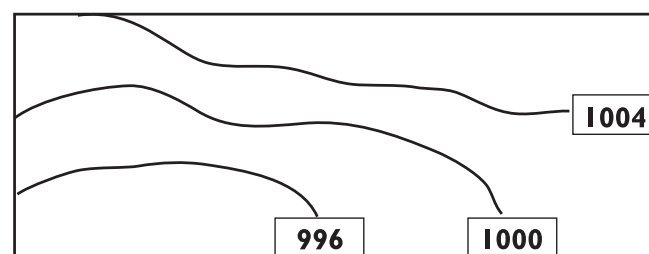
Figure 4.4(g)—Isobars
