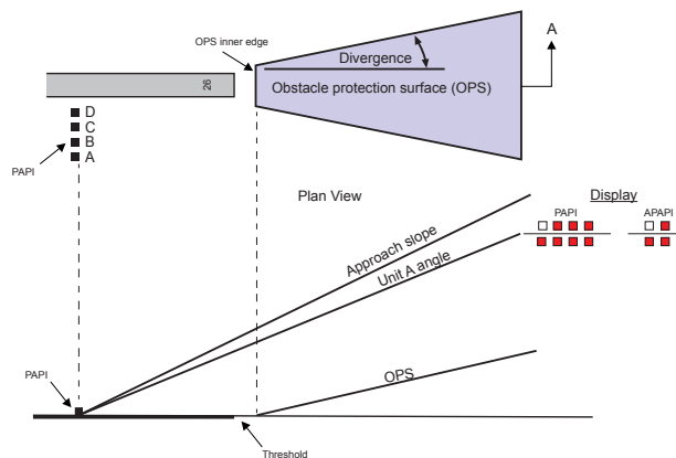
Figure 7.9—PAPI/APAPI OPS
