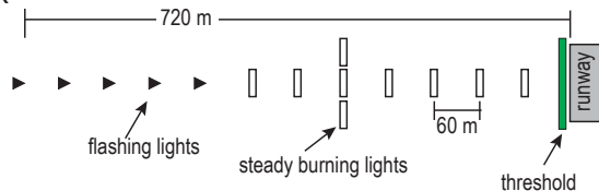
Figure 7.4—MALSR
