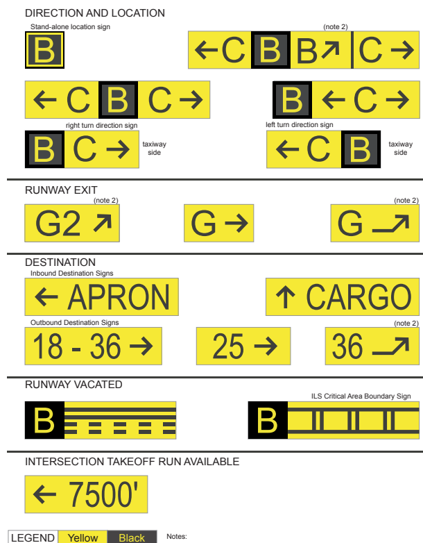
Figure 5.13—Information Signs
