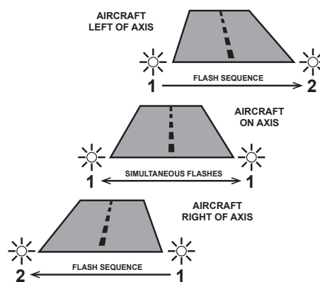
Figure 7.10—VAGS
