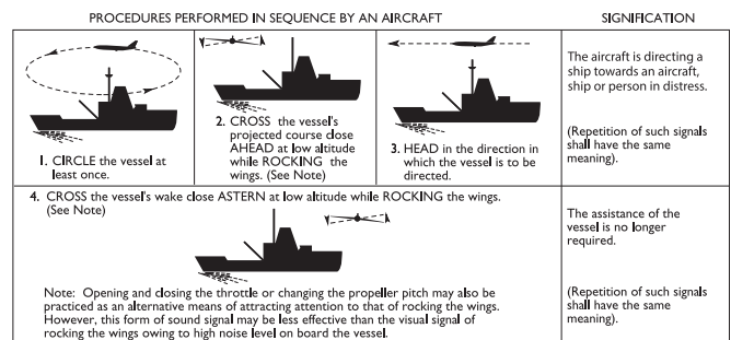
Figure 2.2—Procedures for Signaling Vessels
