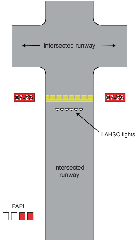
Figure 4.8—LAHSO Visual Aid Configuration
