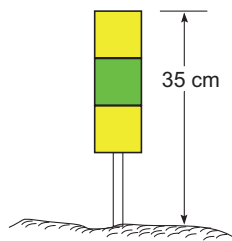
Figure 5.2—Air Taxiway Edge Marker
