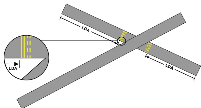
Figure 4.7—Landing Distance Available and Hold Lines for LAHSO
