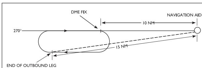
Figure 10.4—DME Hold
