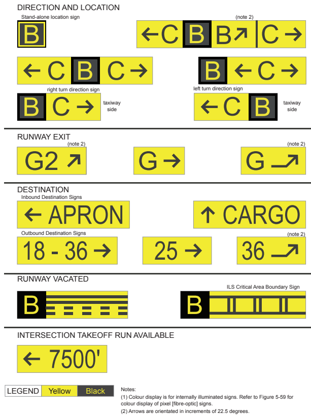
Figure 5.13—Information Signs
