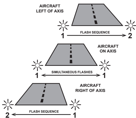
Figure 7.10—VAGS
