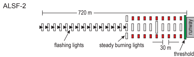
Figure 7.5—ALSF-2
