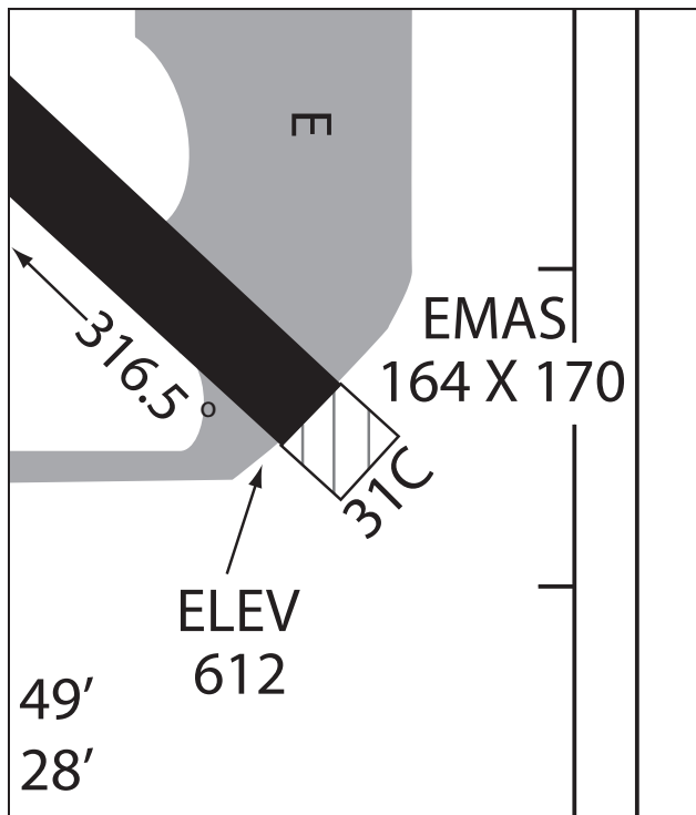
Figure 9.2—EMAS Depiction on an Aerodrome Sketch
