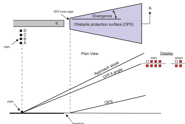
Figure 7.9—PAPI/APAPI OPS
