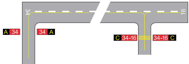
Figure 5.14—Examples of Runway Designation Signs
