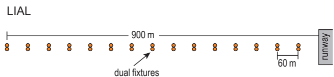
Figure 7.1—LIAL
