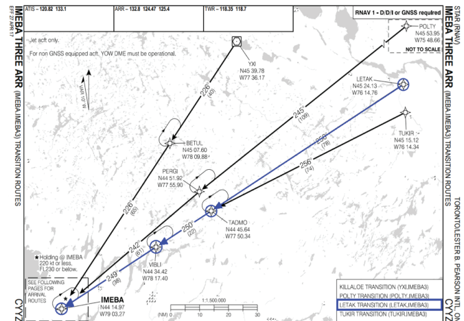
Figure 9.2—Example of an En route Transition on the IMEBA THREE ARR into CYYZ
