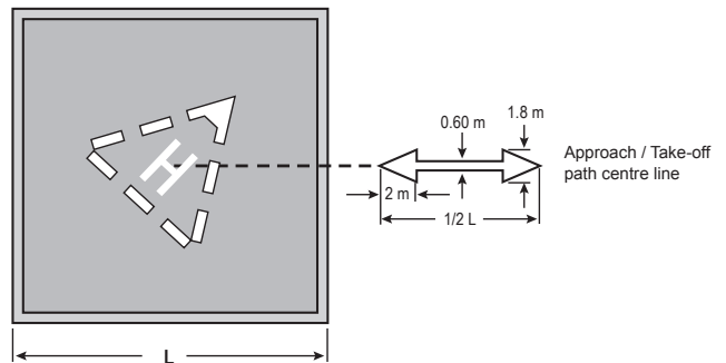
Figure 5.10—Approach and Take-Off Direction Marking
