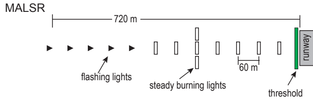
Figure 7.4—MALSR
