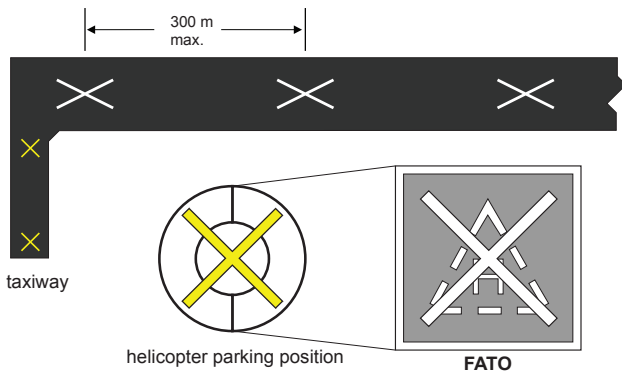
Figure 5.11—Closed Markings
