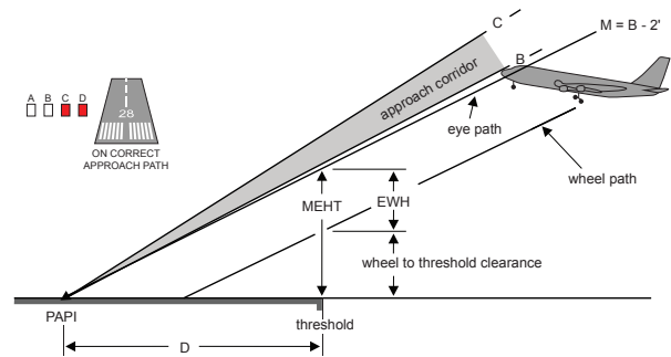
Figure 7.8—PAPI: Pilot Eye Path to Wheel Path
