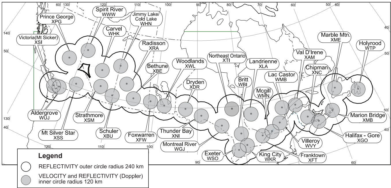
Figure 1.1—ECCC/DND Weather Radar Network
