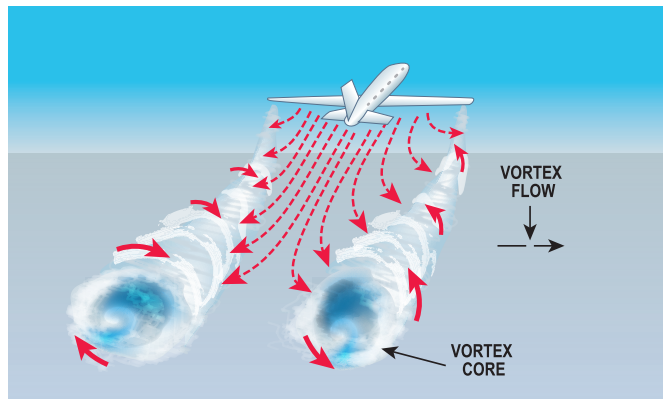
Figure 2.9—Wake Turbulence
