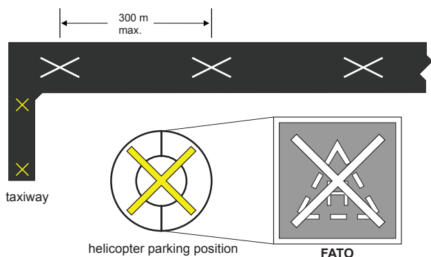
Figure 5.11—Closed Markings
