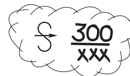
Figure 12.2(g)—Widespread Sandstorms or Dust Storms
