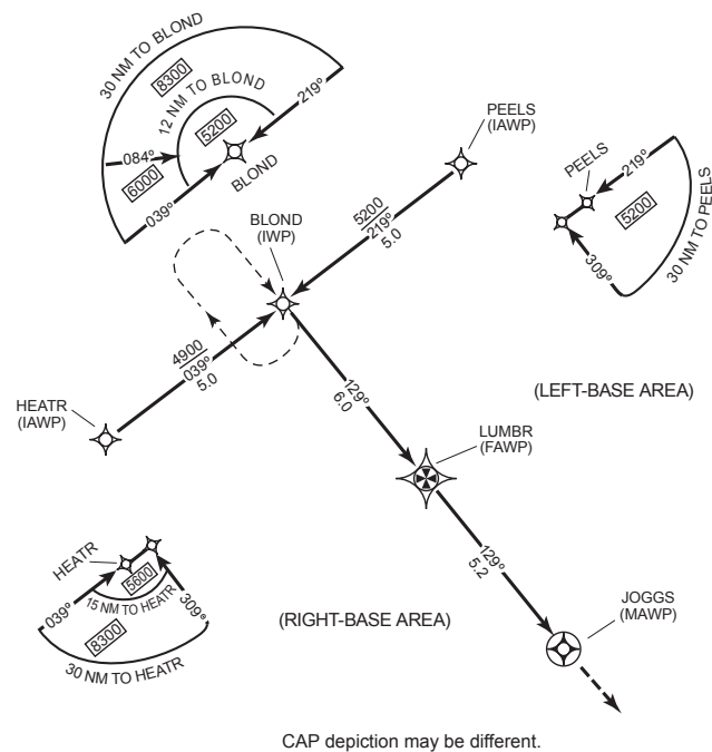
Figure 9.1—Basic “T” Approach with TAA Depiction
