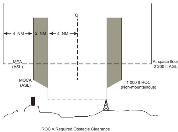
Figure 2.7(b)—Fixed RNAV Route Cross Section
