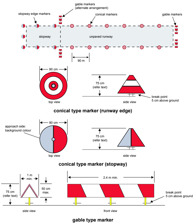
Figure 5.1—Examples of Conical and Gable Markers
