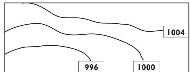
Figure 4.4(g)—Isobars
