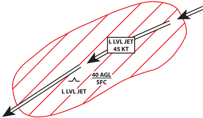
Figure 4.5(i)—Low-level jet and Turbulence
