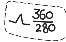
Figure 12.2(e)—Turbulence
