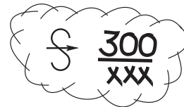
Figure 12.2(g)—Widespread Sandstorms or Dust Storms
