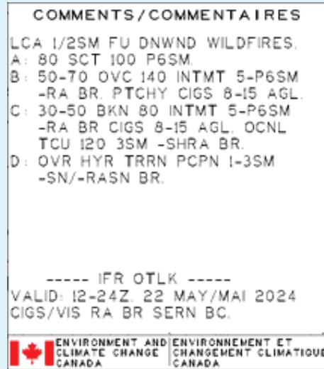
Figure 4.3—GFA Comments Box
