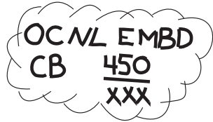
Figure 12.2(b)—Clouds Heights
