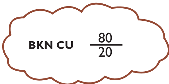
Figure 4.4(c)—Organized Area of Clouds (scalloped border)
