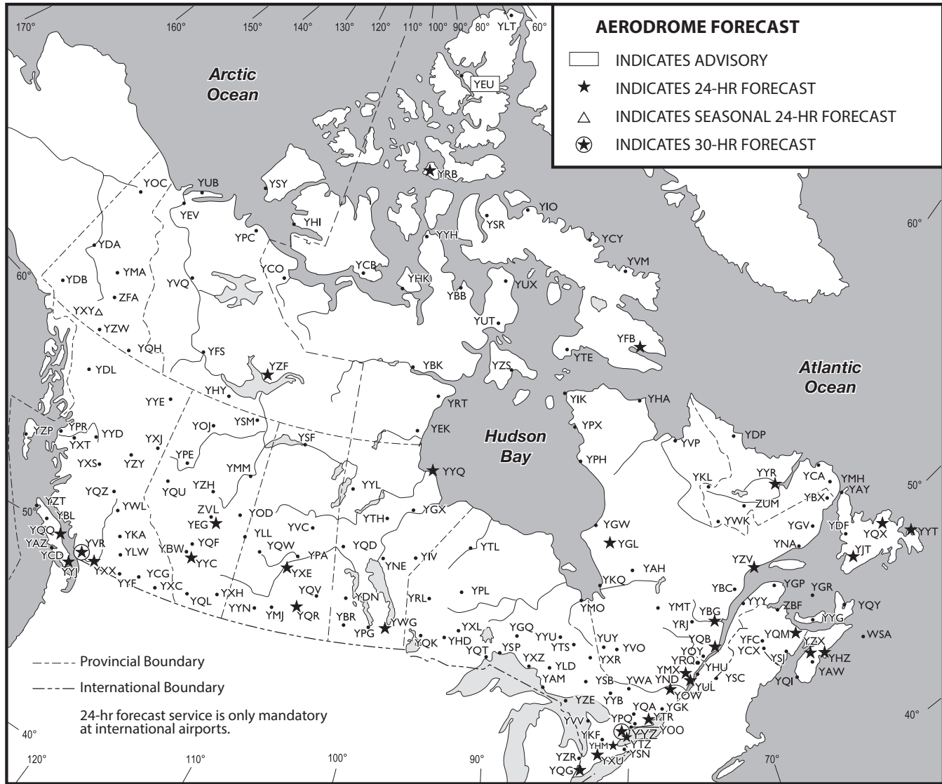
Figure 7.1—TAF Locations
