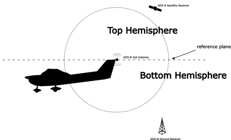
Figure 4 - Top and Bottom Transmission Hemispheres – Single Antenna
