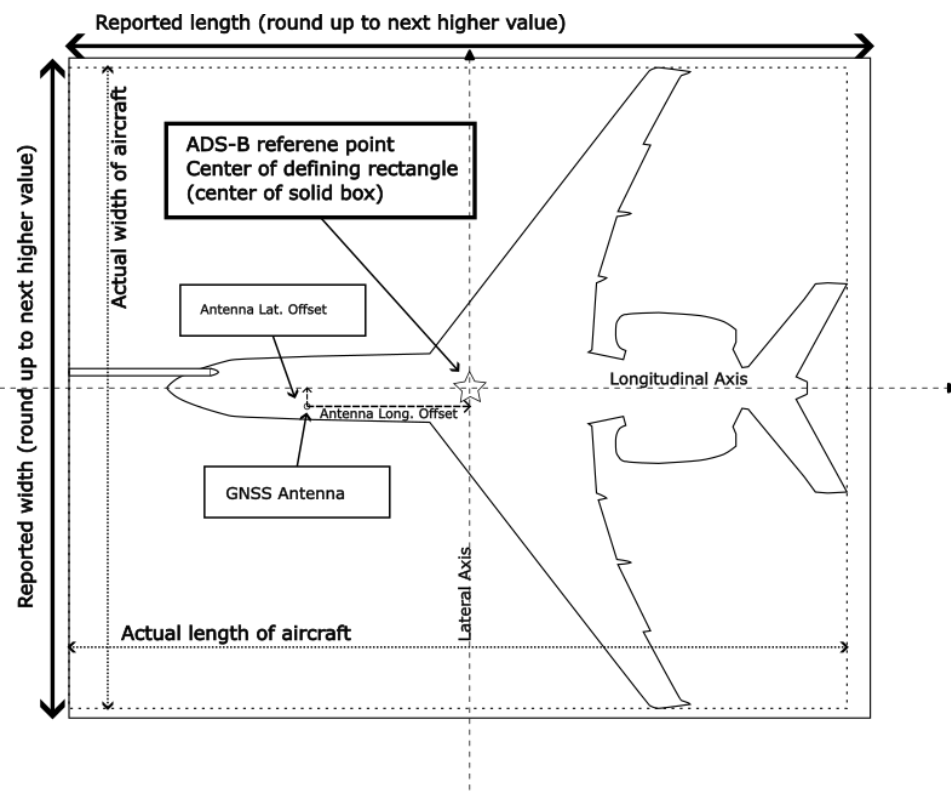
Figure 2 - A/C length, width and antenna offset
