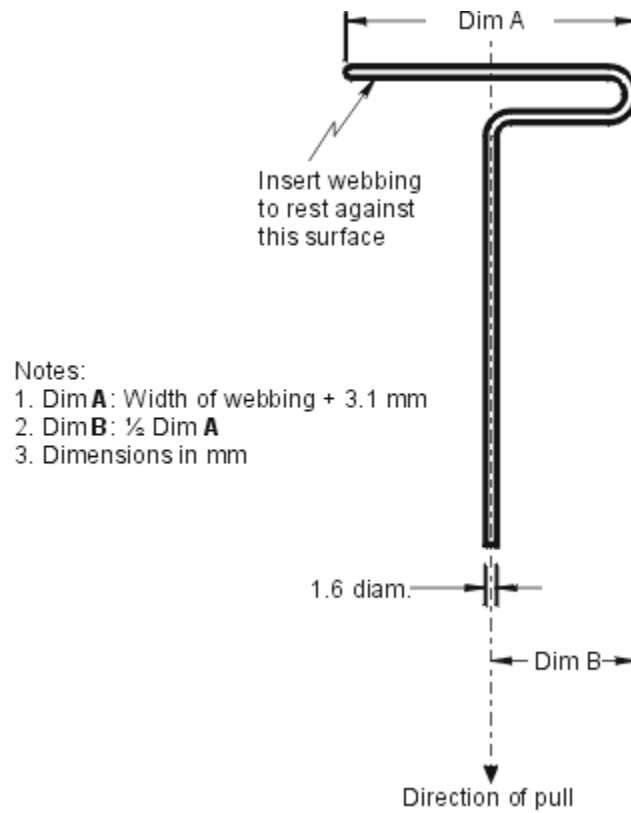
Figure 5 — Webbing Tension Pull Device
