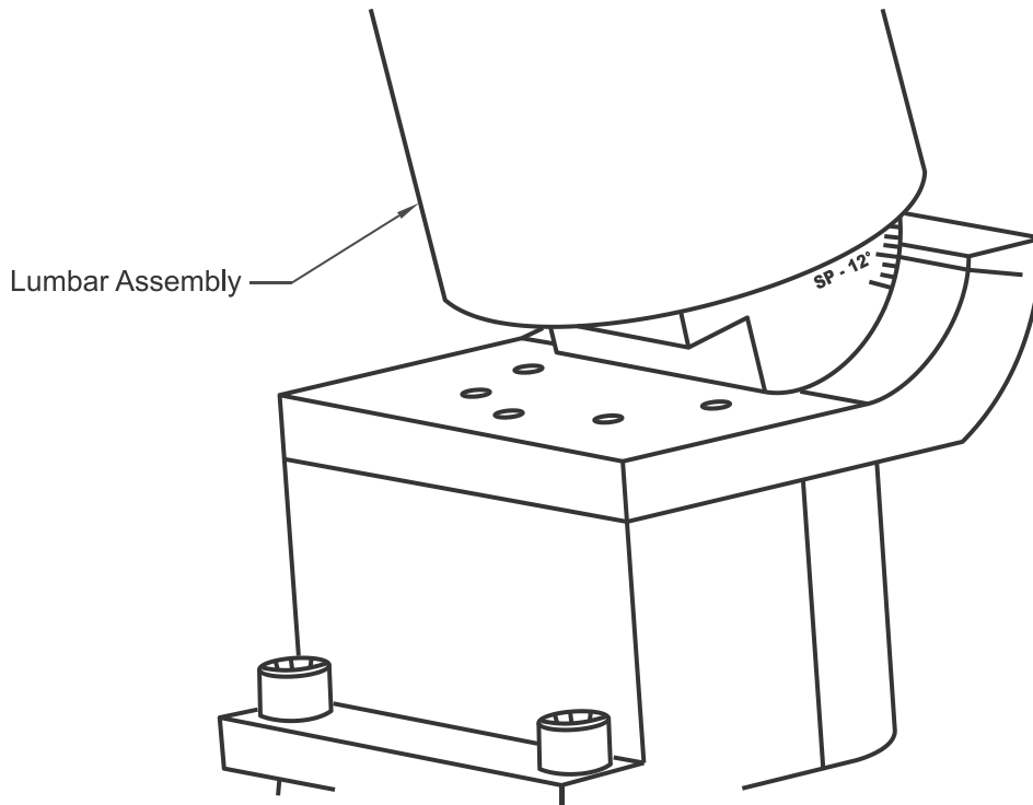
Figure 8 — HIII-10C Dummy Lumbar Angle Setting is SP-12 Degrees
