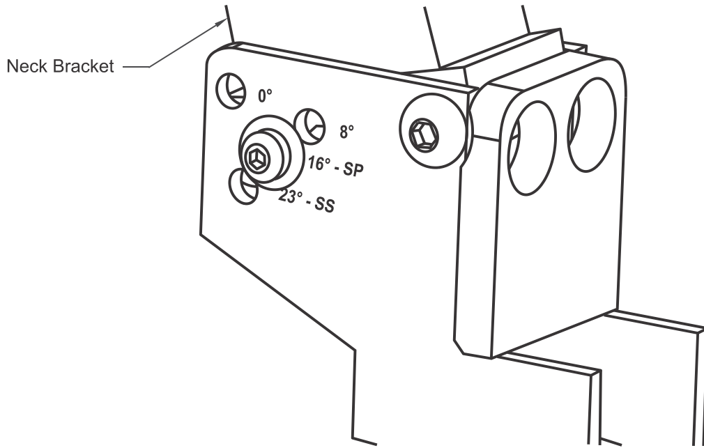
Figure 7 — HIII-10C Dummy Neck Angle Setting is SP-16 Degrees
