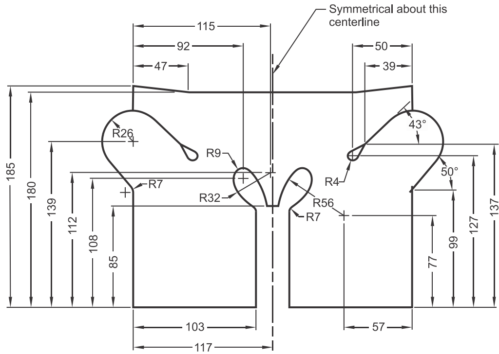
Figure 6 — Lap Shield
