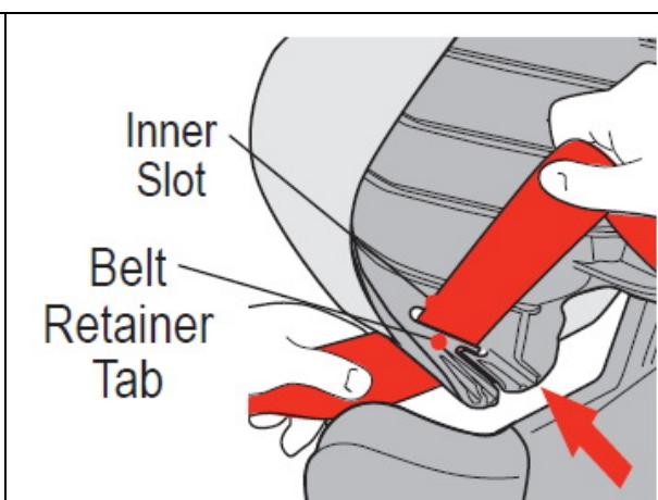
Figure 3. Z-Shaped Shoulder Belt Guide
