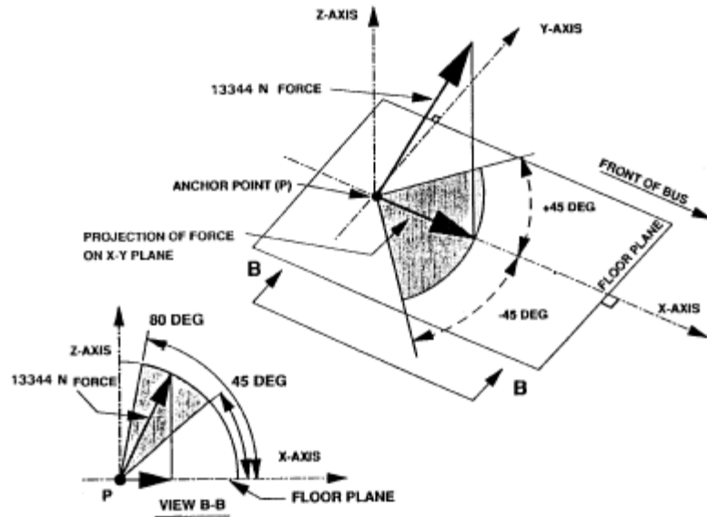
Figure 5. Pelvic Restraint Anchorage Loading Direction
