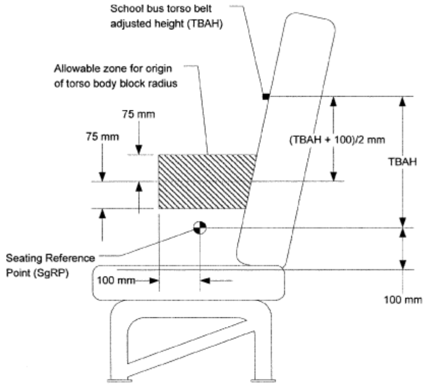
Figure 9 – Torso Block Zone
