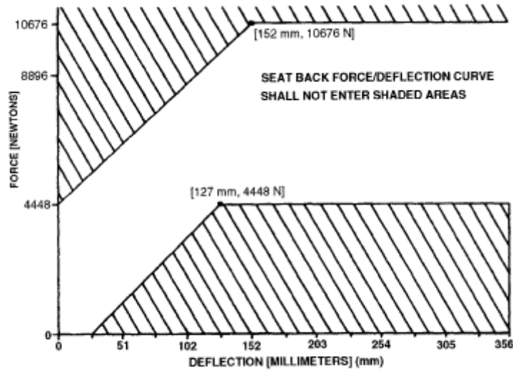
Figure 1.—Force/Deflection Zone
