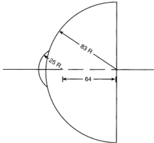
Figure 3 All dimensions in millimeters (mm)
